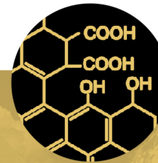
Fulvic Acid
